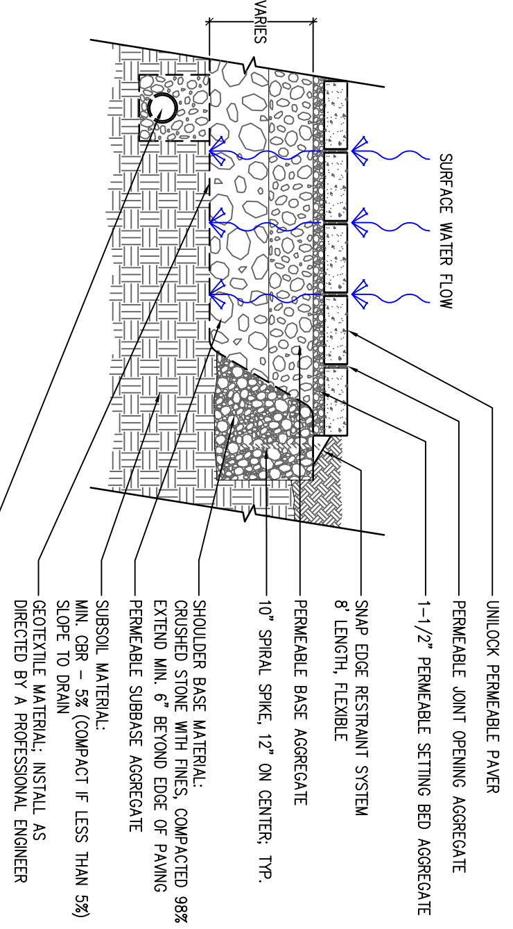
12 Permeable Pavers with Shoulder CS-COM-PERM-SHOULDER
